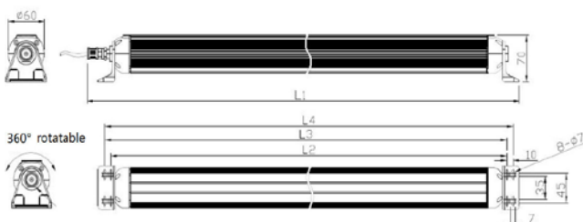
Abmessungen M9R (in mm)
